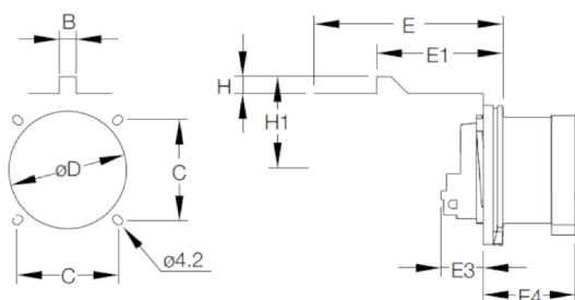
Dimensions (mm)
