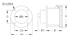
Dimensions (mm)
