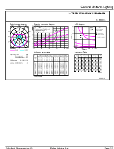
General uniform lighting - CorePro LEDtube UN 1500mm UO 23W865 T8
