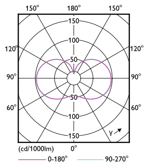
Light Distribution Diagram - TForce Core LED HPL 36W E27 827 FR
