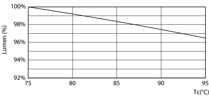
Lumen Maintenance Diagram - MAS LEDtube HF 1500mm UO 36W 840 T5
