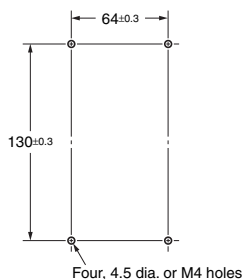
Four, 4.5 dia. or M4 holes
