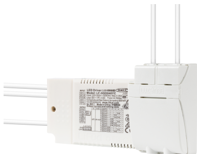
Driver DALI 2 700mA m/Linect 5P
