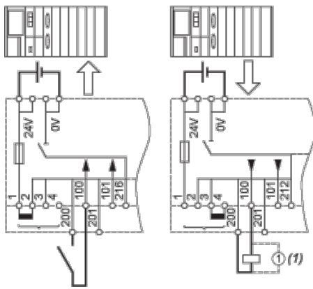
(1) Inductive load
