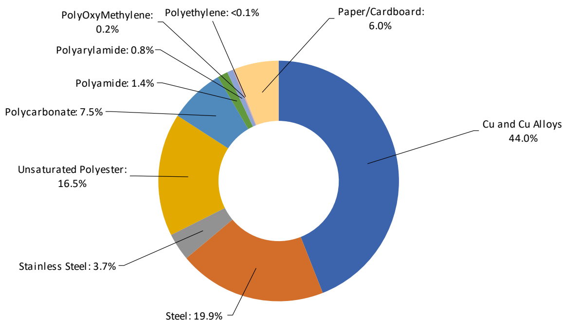
Figure 1: Composition of XT6 W FP 3P HR/HR IEC/UL
