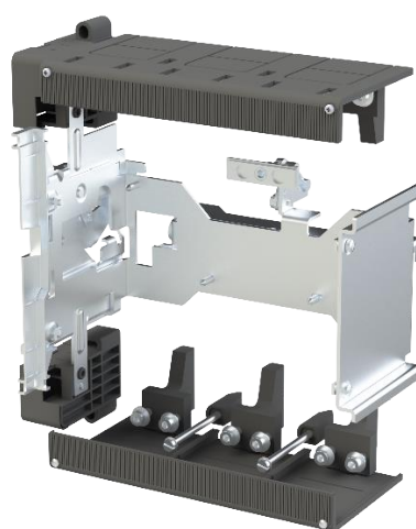
XT6 W Conversion Kit
