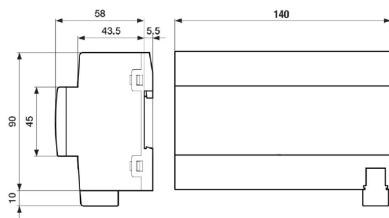
Dimension drawing
