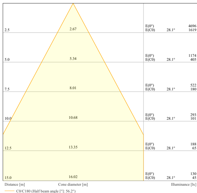
FL FLEX DA/P 180W ML 840 R60 WAL
