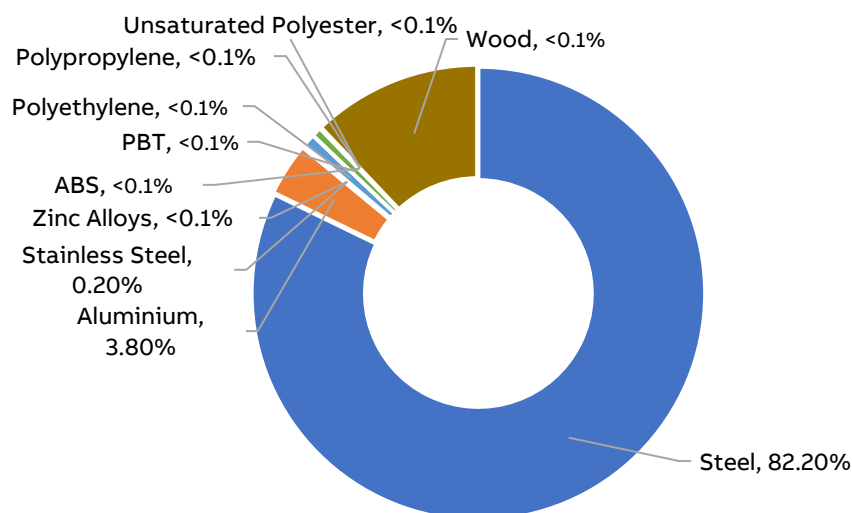
Figure 1: Composition of CDC640 NO Cabinet
