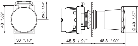
MPET4 Dimensions (mm, inches)
