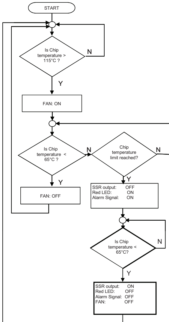
ALARM Signal and Fan (applicable to RGC..D92GGEP)
