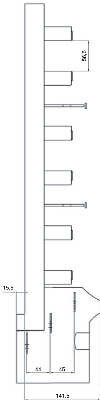
Dimensions (mm) - EBF 00 185 mm busbar system
