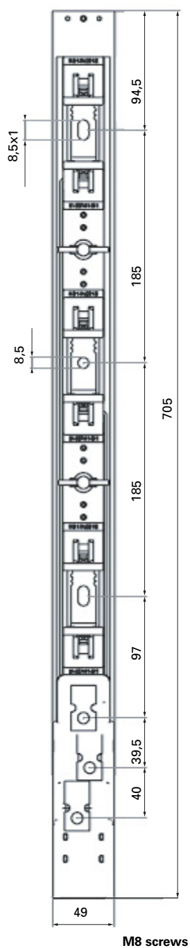
Dimensions (mm) - EBF 00 185 mm busbar system
