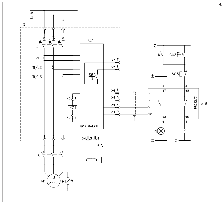
Ekip M-LRIU electronic trip unit connected to PR212/CI contactor control unit
