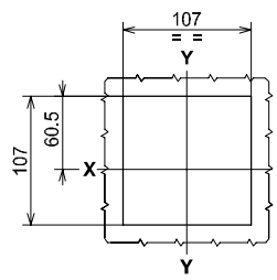
Without flange
