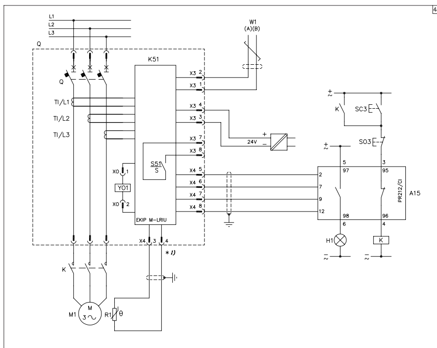
Ekip M-LRIU electronic trip unit with auxiliary supply connected to PR212/CI contactor control unit with MODBUS RS485 communication option
