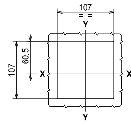
Without flange
