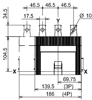
Front extended 400 A - EF
