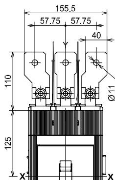
Front extended spread 630 A - ES
