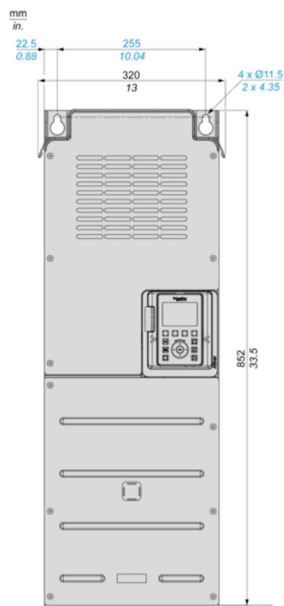
Drives with Lower Conduit Box Sold Separately Rear, Front and Left View
