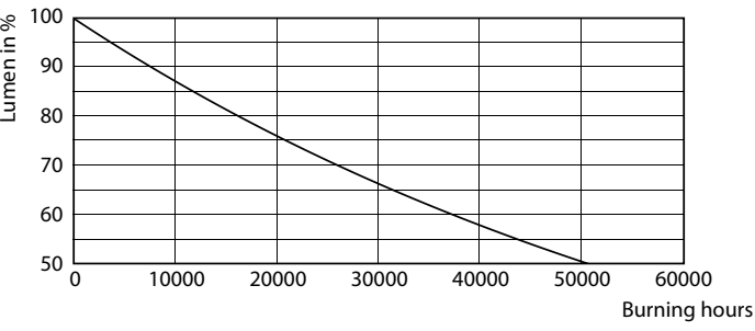
Lumen Maintenance Diagram - CorePro LED HPI MV 15Klm 105W840E40 100D
