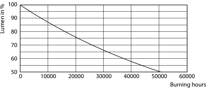
Lumen Maintenance Diagram - TForce Core LED HPL 36W E40 827 FR
