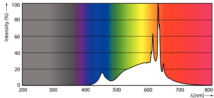
Spectral Power Distribution Colour - MAS VLE LEDBulb D7.8-75W E27 927 A60 FRG
