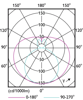
Light Distribution Diagram - CorePro LEDtube UN 1200mm UO 15.5W840 T8
