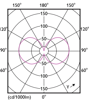
Light Distribution Diagram - MAS LEDBulbND5.2-75W E27 840 A60 CL G UE
