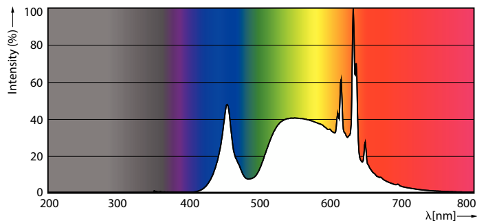
Spectral Power Distribution Colour - MAS LEDBulbND5.2-75W E27 840 A60 CL G UE
