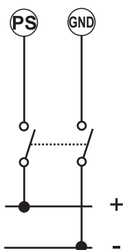
Fig. 7 Power supply
