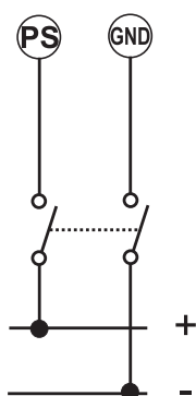
Fig. 11 Power supply
