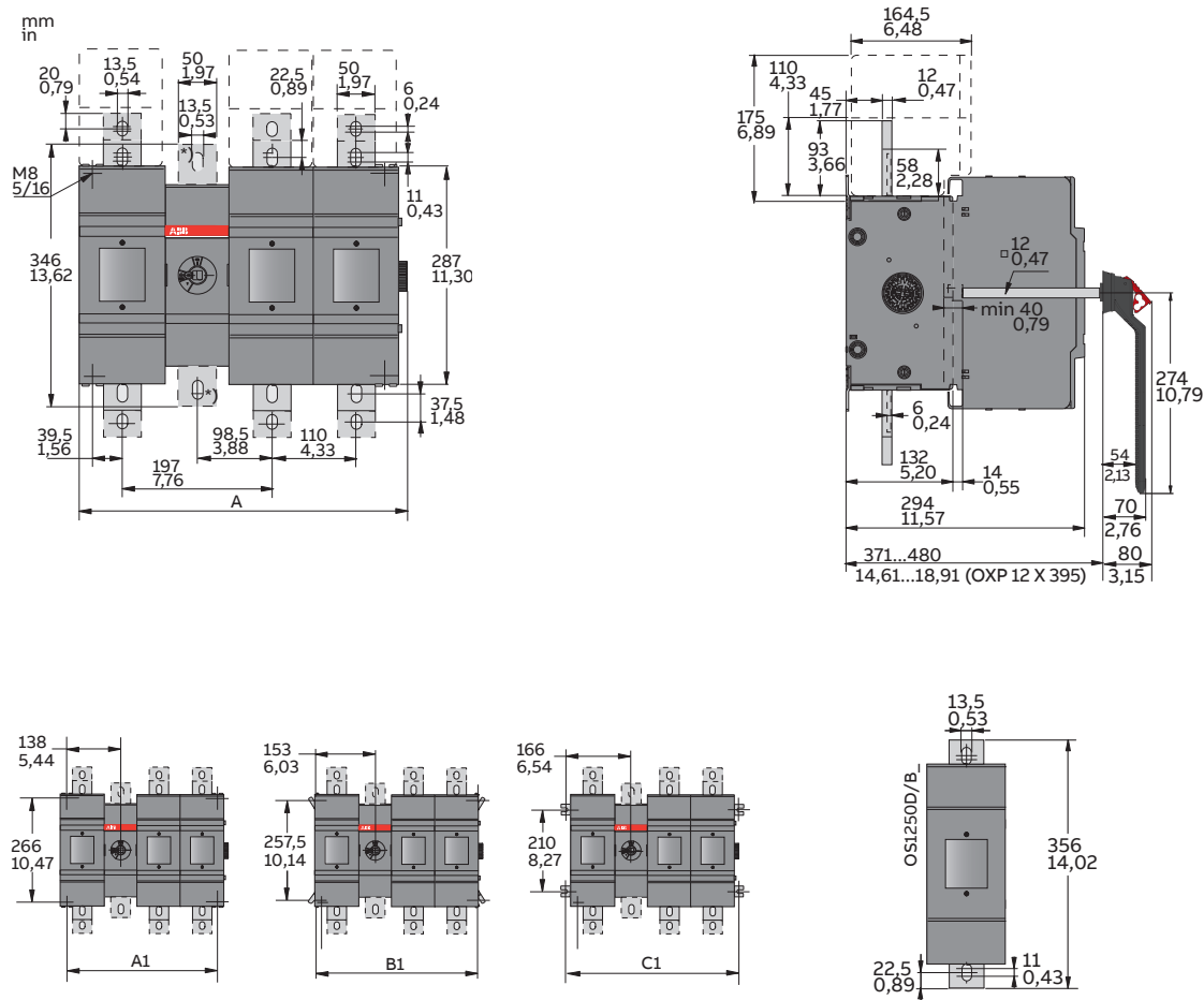
OS1200...1250_P Mechanism between the poles
