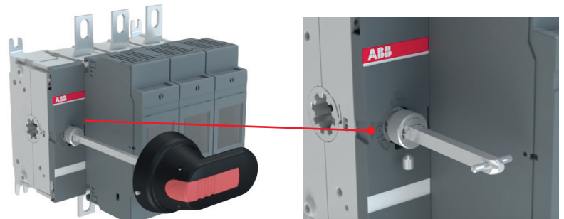
Adjustable shaft
