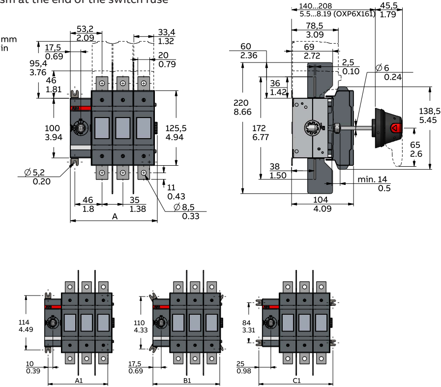
OS100GJ_ Mechanism at the end of the switch fuse
