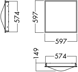
C90-R625X625 DROP OUT
