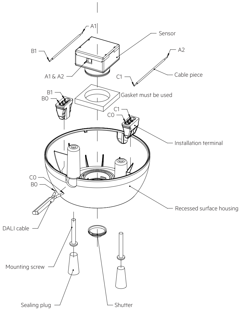
Exploded view
