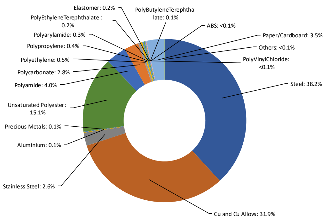
Figure 1: Composition of E1.2 B-A/N-A/S-A 1200A UL 3P
