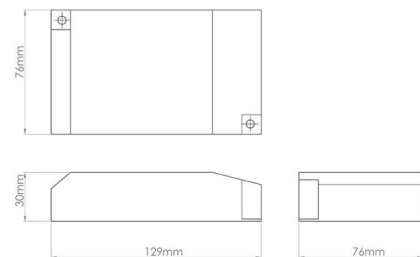
SENSE 1400mA /5000lm DRIVER DALI
