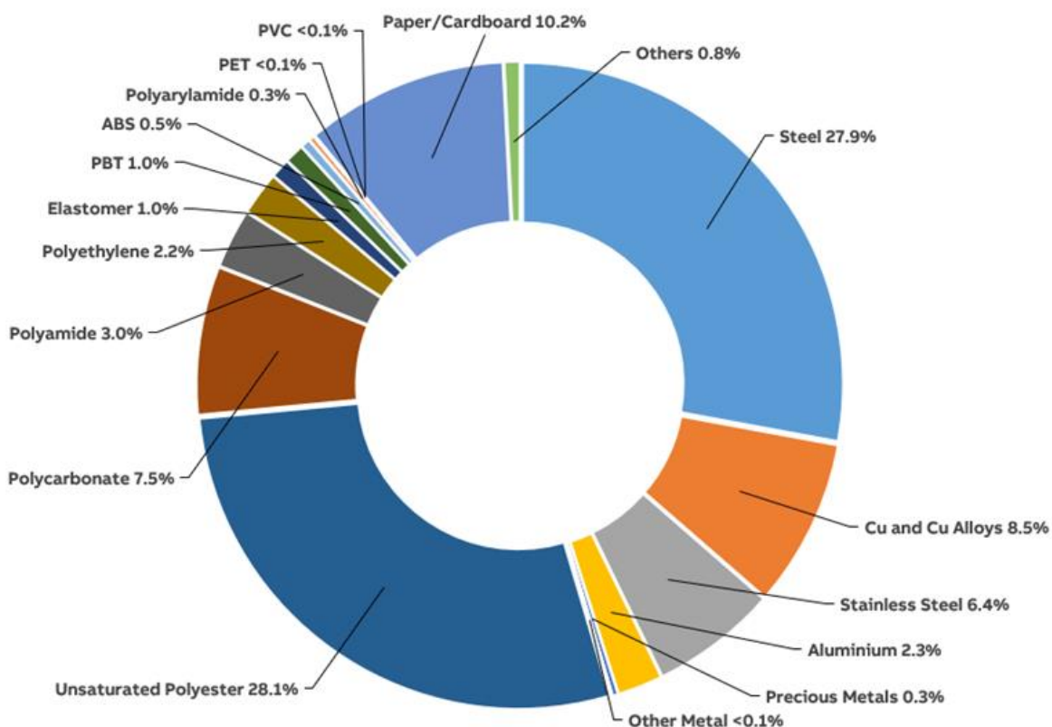
Figure 1: Composition of XT5 3p IEC N/S/H/L Ekip DIP 400A
