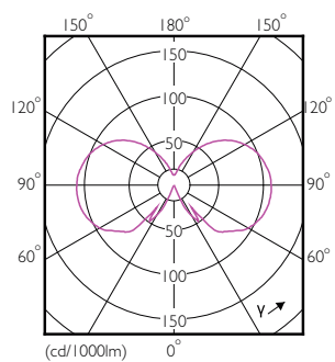
LEDbulb 40W E27 827 CL A60 DT
