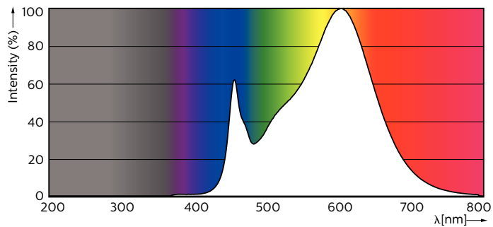
LEDtube 1200mm HO 14W830 T8
