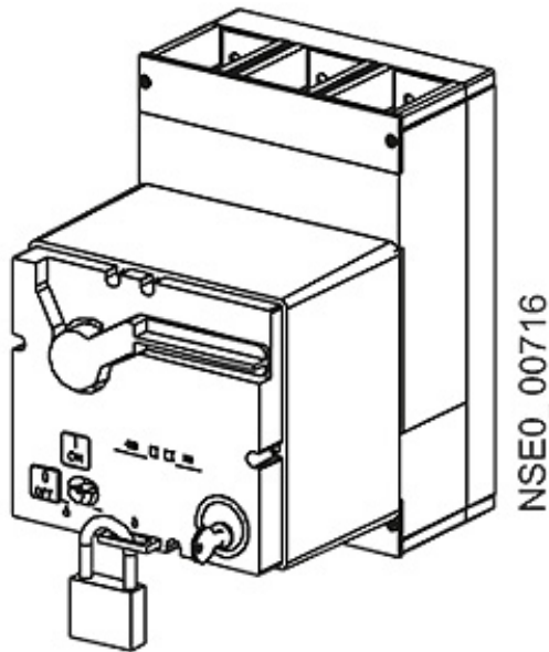
ACCESSORY FOR VL400, STORED ENERGY OPERATOR 24V DC
