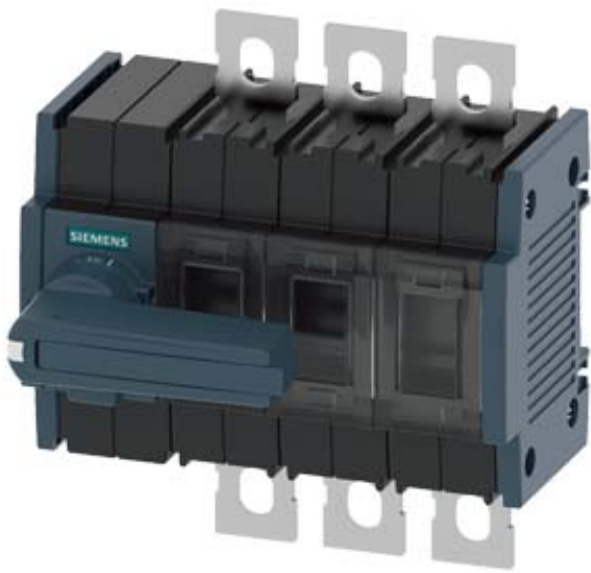
SWITCH-DISCONNECTOR 200A, FRAME SIZE 3, 3-POLE FRONT OPERATING LEFT COMPLETE ASSEMBLY WITH DIRECT HANDLE GREY FLAT TERMINAL INCL. PHASE BARRIERS
