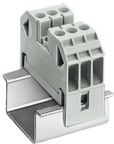
THROUGH-TYPE TERMINAL THERMOPL. SCREW TERMINAL ON BOTH ENDS TERMINAL BLOCK 3-POLE, BEIGE 19.5MM, SZ. 4
