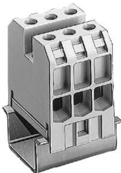
THROUGH-TYPE TERMINAL THERMOPL. SCREW TERMINAL ON BOTH ENDS BLOCK 3 TERMINALS 30.2MM, SZ16
