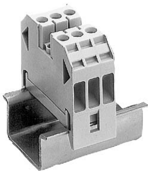
THROUGH-TYPE TERMINAL THERMOPL. SCREW TERMINAL ON BOTH ENDS TERMINAL BLOCK 3-POLE, BEIGE 24.5MM, SZ. 6
