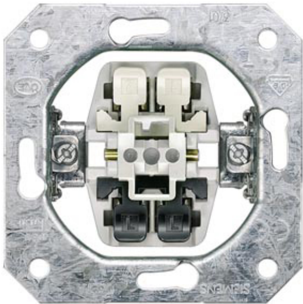
DELTA SWITCH INSERT FM OFF SWITCH 2POLE 10A 250V
