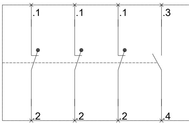
3RT2
