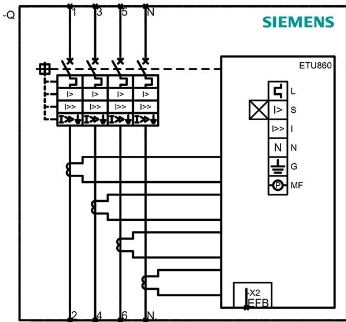
Internal circuit diagram IEC
