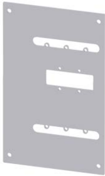
REAR INTERLOCK MOUNTING PLATE ACCESSORY FOR: 3VA2 100/160/250 3VA6/7 150/250
