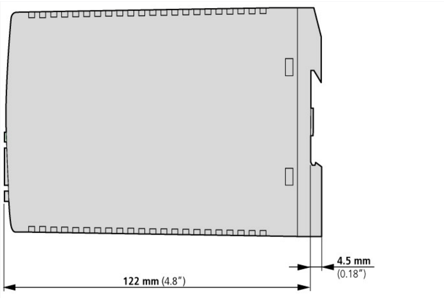
SmartWire-DT Gateways
