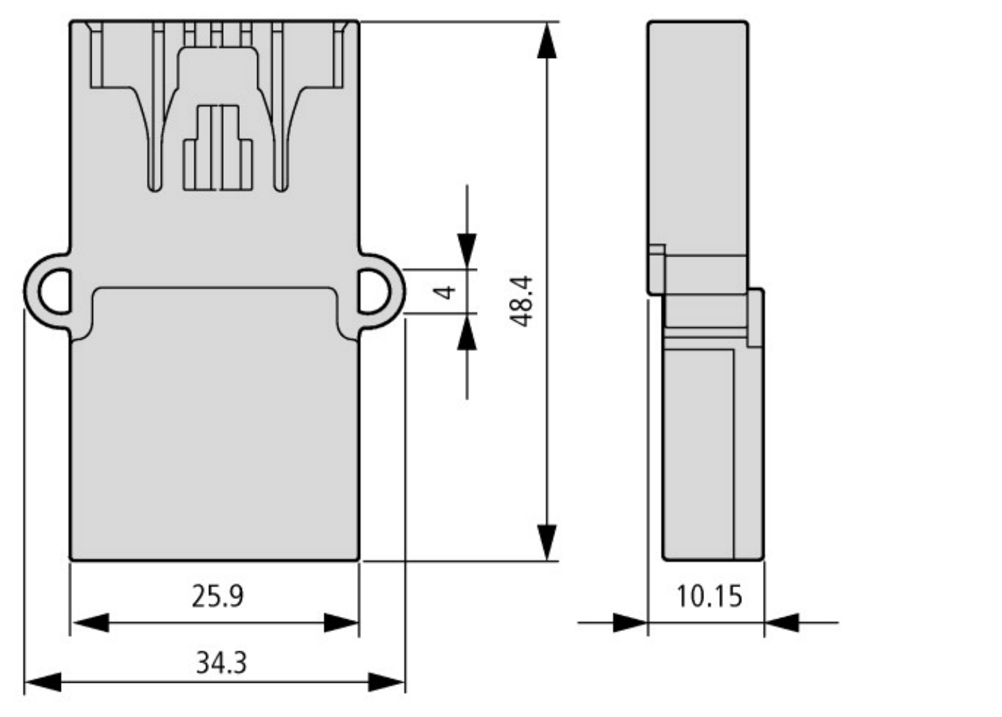
Bus termination Network terminator
