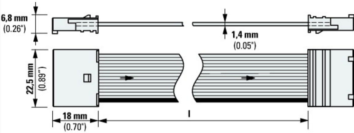
SWD ribbon cable
