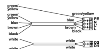
Through-wiring set
