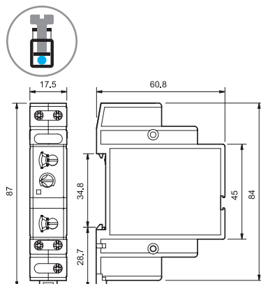
Type 80.82 Screw terminal
