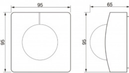
IS 3360 MX Highbay
