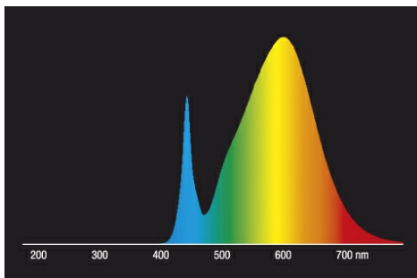
LED retrofit standard lamps 25W replacement, 2700K
