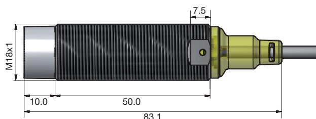
Fig. 17 Long body, non-flush version, cable
