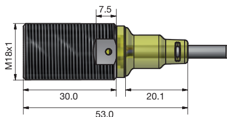
Fig. 12 Short body, flush version, cable
