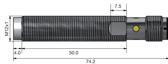
Fig. 11 Long body, non-flush version, plug
