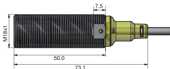
Fig. 16 Long body, flush version, cable
