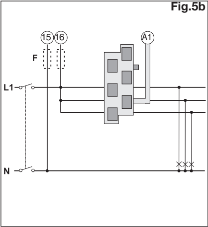
1-ph. system type selection 3.1P
