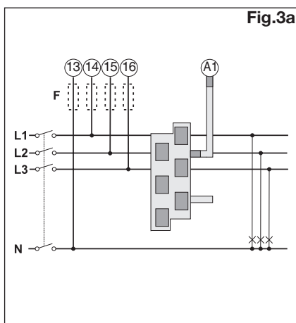
3-ph. system type selection 3.1P
