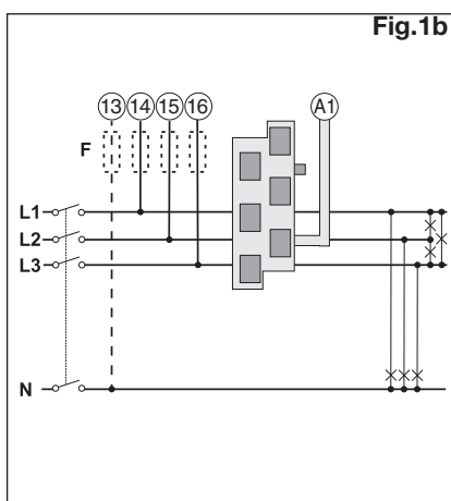
3-ph. system type selection 1.3P
