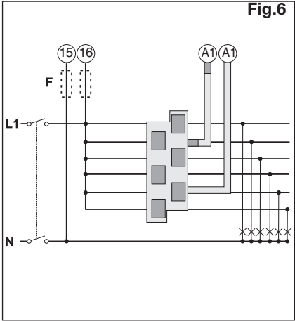
1-ph. system type selection 6.1P
