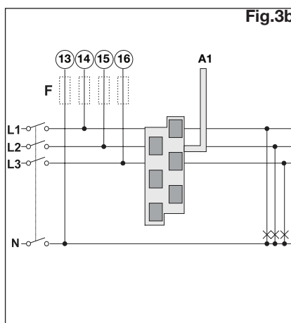
3-ph. system type selection 3.1P
