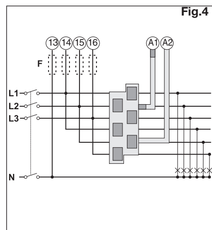
3-ph. system type selection 6.1P
