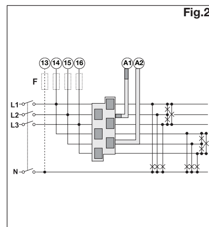
3-ph. system type selection 2.3P
