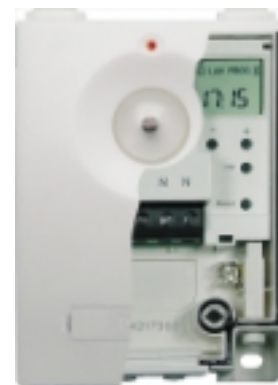
Luna 129
